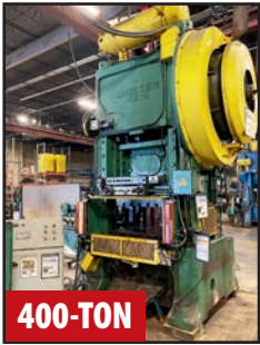
MINSTER 40E-9 STRAIGHT SIDE PRESS W/FEED AND STRAIGHTENER
