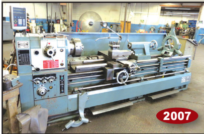
KINGSTON HD2290 Gap Bed 22/31-3/8" x 90" Engine Lathe
