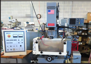
HANSVEDT CS-1 Ram Type EDM w/Pulse PS
