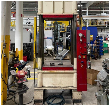
75 TON KR WILSON 4 POST HYDRAULIC SPOTTING PRESS
