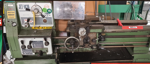
JET 1430 LATHE
