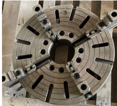
25" 4 2 PIECE JAW CHUCK 6 1/2" THRU HOLE
