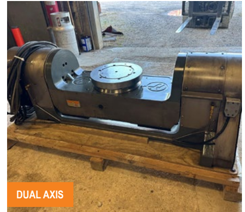
DUAL AXIS HAAS TR310 DUAL AXIS TRUNNION ROTARY TABLE
