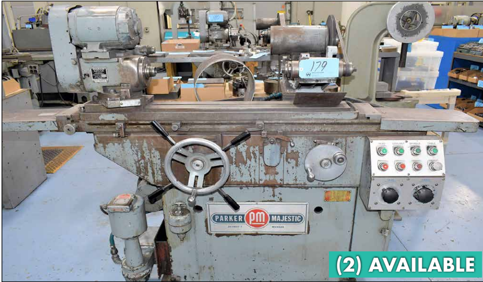
Parker Majestic ID Grinder, Parker Model 2300-3 Spindle
