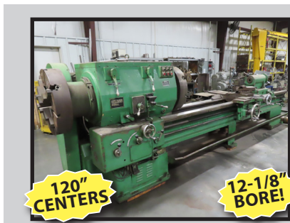
LEHMANN BIG HOLE LATHE
