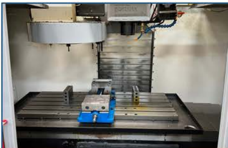
2013 Creative Evolution HSD-500 Vertical Milling Machine
