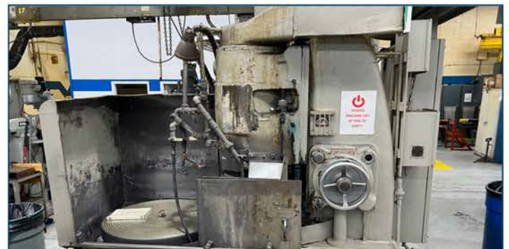
Blanchard #18 Rotary Surface Grinder: 18" Diameter Grinding Wheel and 36" Magnetic Chuck
